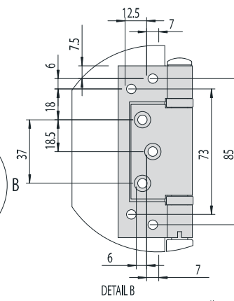
Intermediate hinges
