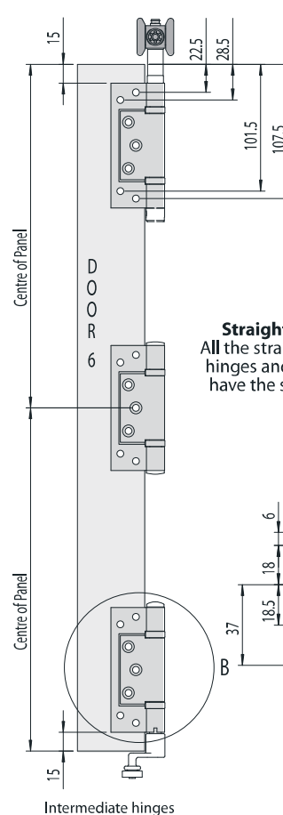
Intermediate hinges
