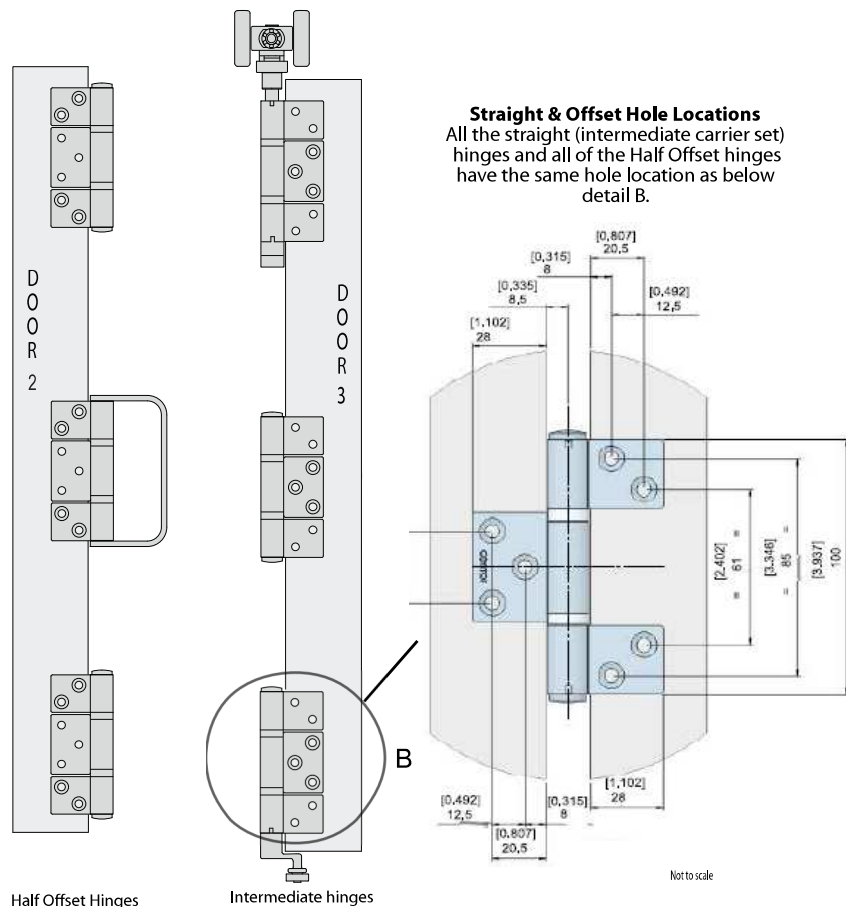
Half Offset Hinges
