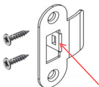
Adjustable latch plate
