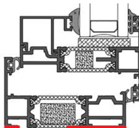
Silicone Seal
