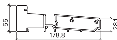
FRAME CILL
