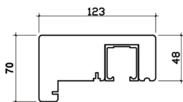
FRAME HEAD
