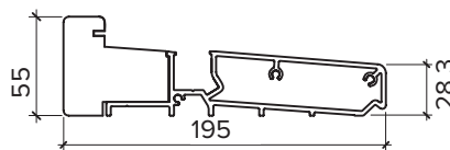
FRAME CILL
