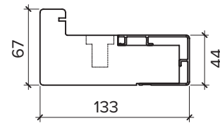
FRAME JAMBS R/L
