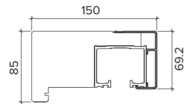
FRAME HEAD
