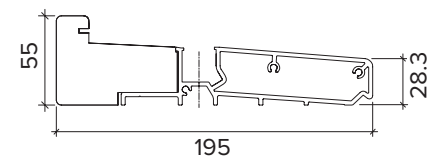
FRAME CILL
